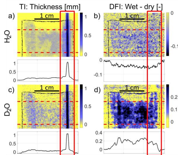
Figure 1: Color coded images showing the water distribution in a GDL (Freudenberg H2315): yellow = dry, blue = water present. [a,c]: Water thickness images calculated from transmission images (TIs): a) H 2 O, c) D 2 O. [b,d]: Difference of DFIs between dry and water filled GDL: b) H 2 O, d) D 2 O. The dashed red lines in the images indicate the area for which the profile is plotted below the images.
